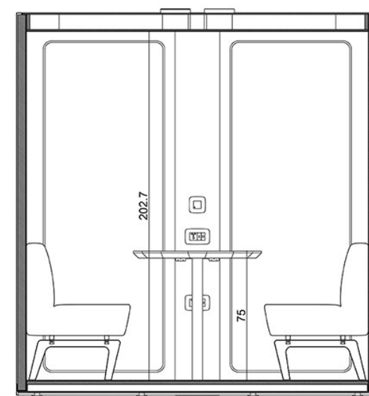
BUSYPOD Large Section
